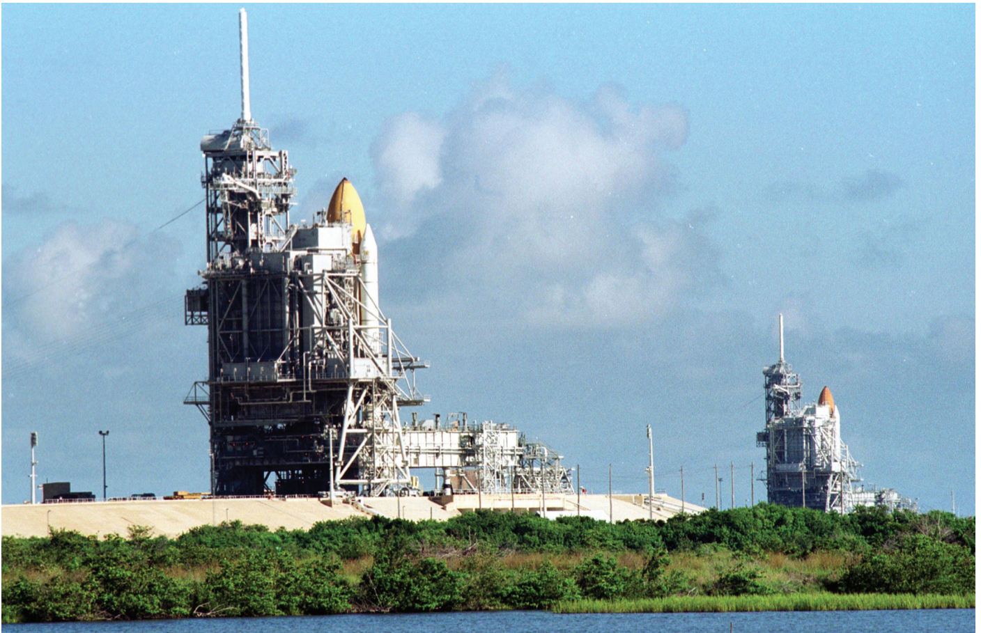
Space Shuttle Discovery (left) and Space Shuttle Atlantis (right) both stand ready on their Launch Pads (39A and 39B respectively). Atlantis launched first, July 12, 2001, on mission STS-104. Discovery launched Aug.10, 2001, on mission STS-105. Towering above each Shuttle at left is an 80-foot-tall lightning rod, part of the lightning protection system at the pads.
